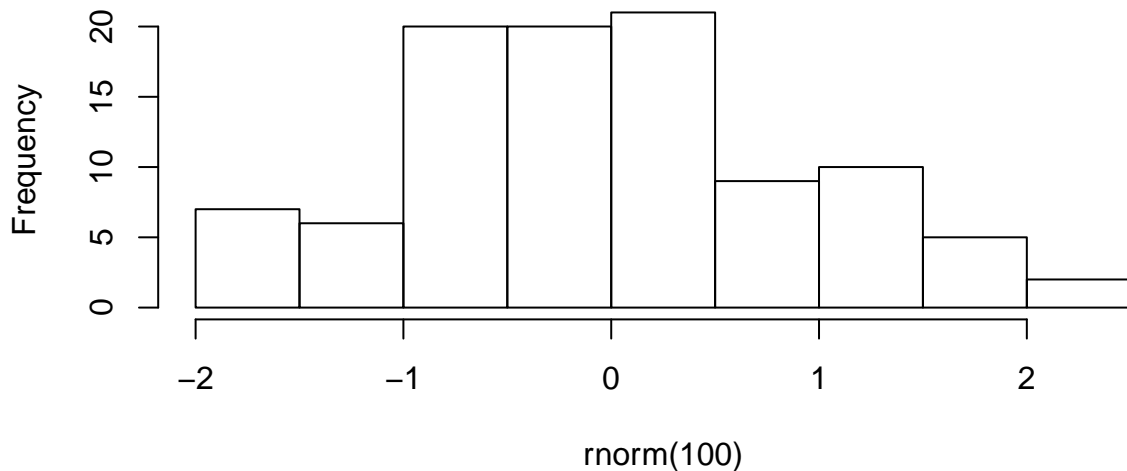
Histogram of rnorm(100)
